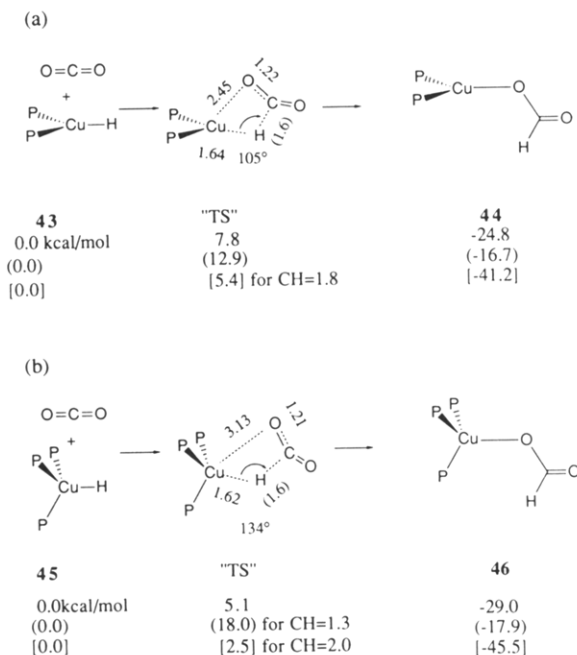
Figure 6. Potential energy profiles for CO 2 insertion to (a) CuH(PH 3 ) 2 ( 43 ) and (b) CuH(PH 3 ) 3 ( 45 ) calculated in kcal/mol at the RHF-ECP level, the MP2-ECP level (in round brackets) and at the all-electron RHF level (in square brackets), relative to the reactants. 65 The "transition state" structures (in angstroms and degrees) are those on the RHF-ECP potential energy curve and are optimized with the C-H distance fixed to be 1.6 Å. At the levels of calculation where the C-H distance at the corresponding TS is not 1.6 Å, the C-H distances are shown together with the activation energies.
