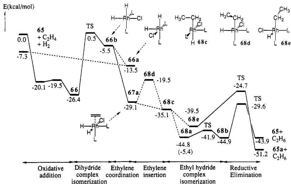
Figure 11. Potential energy profile of the catalytic cycle of the Brown mechanism of olefin hydrogenation by the Wilkinson catalyst, in kcal/mol at the RHF-ECP level, relative to 65 + H_2 + C_2H_4 . 107
