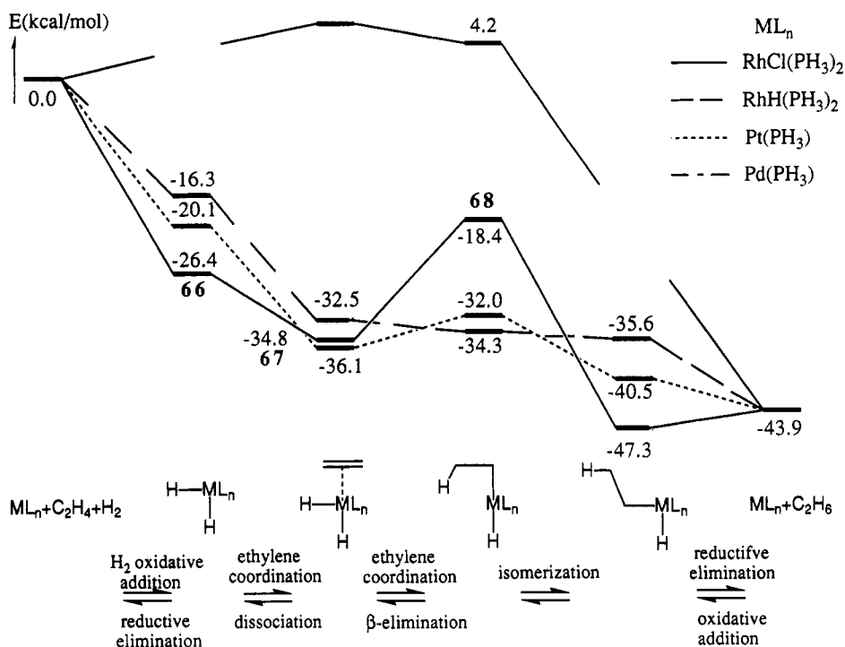
Figure 10. Energy changes (in kcal/mol) of the full hydrogenation cycle by RhCl(PH_3)_2 , RhH(PH_3)_2 , Pd(PH_3) , and Pt(PH_3) . The profiles show only the energies of intermediates but not those of transition states connecting them. 12
